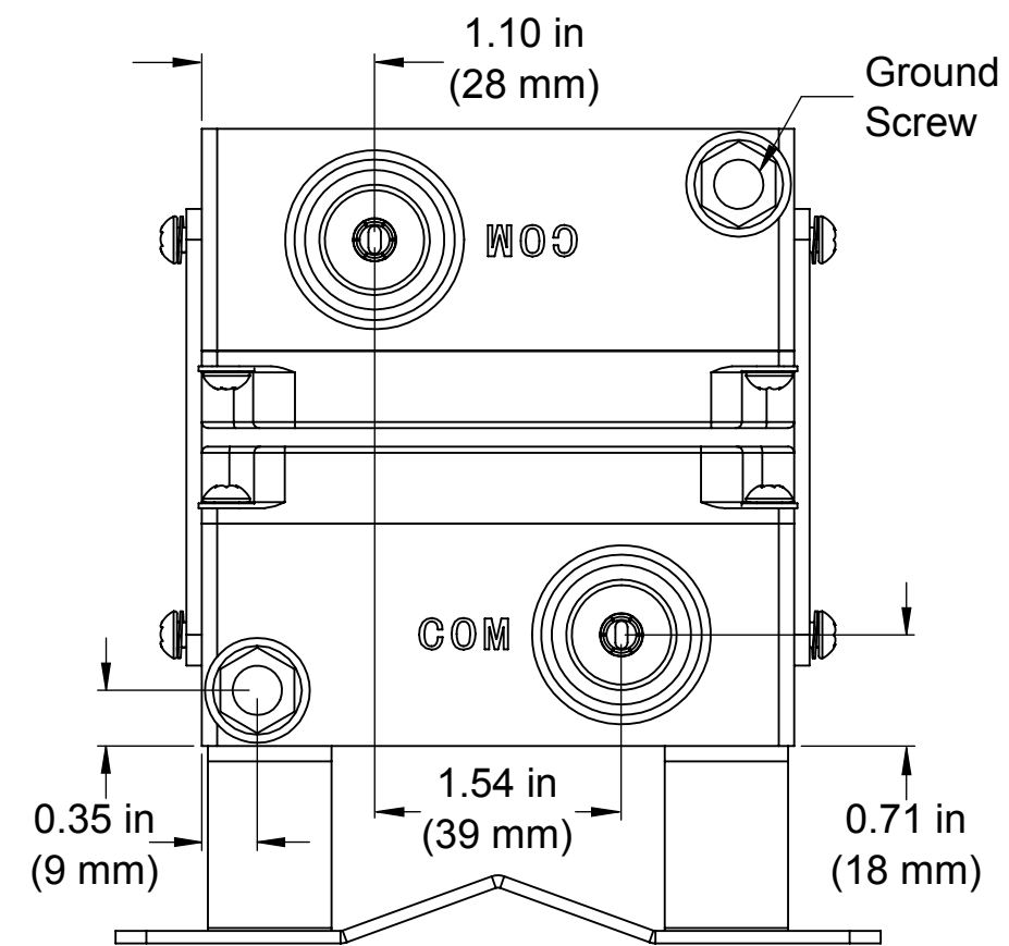
Double diplexer configuration common port view
