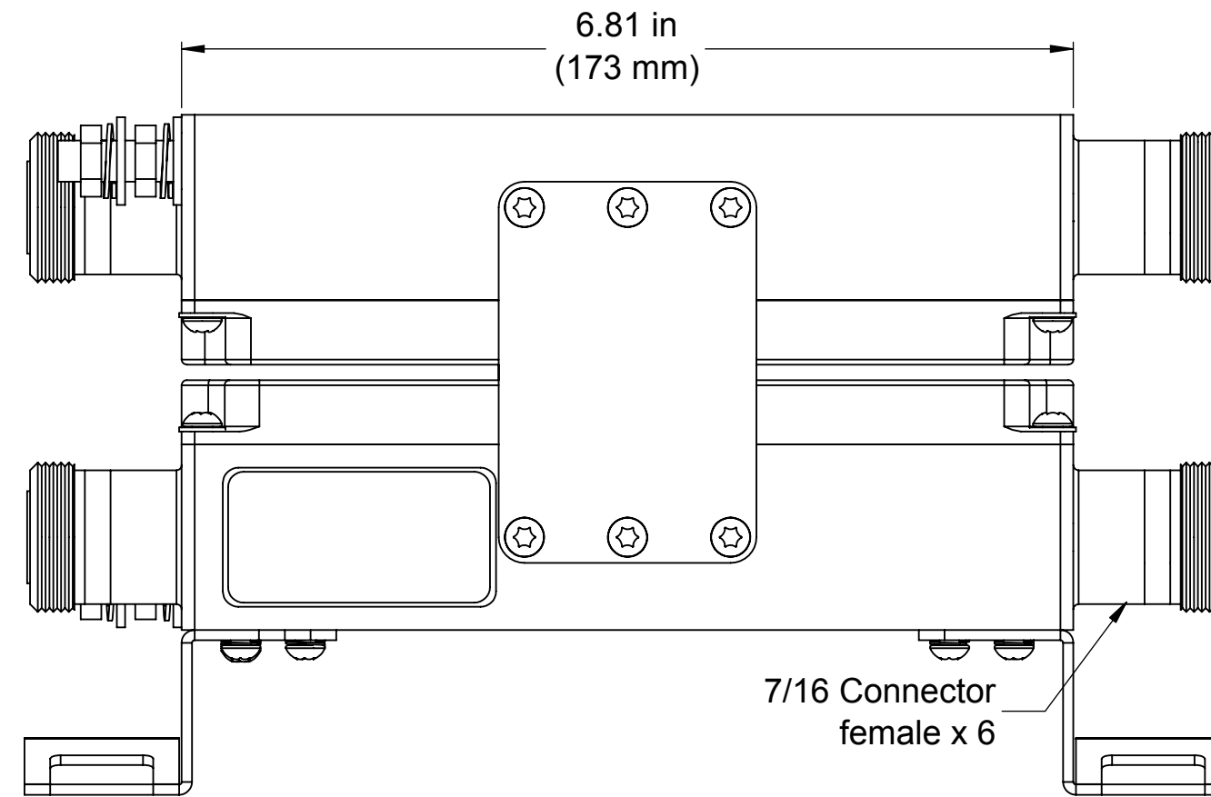
Double diplexer configuration side and bottom views
