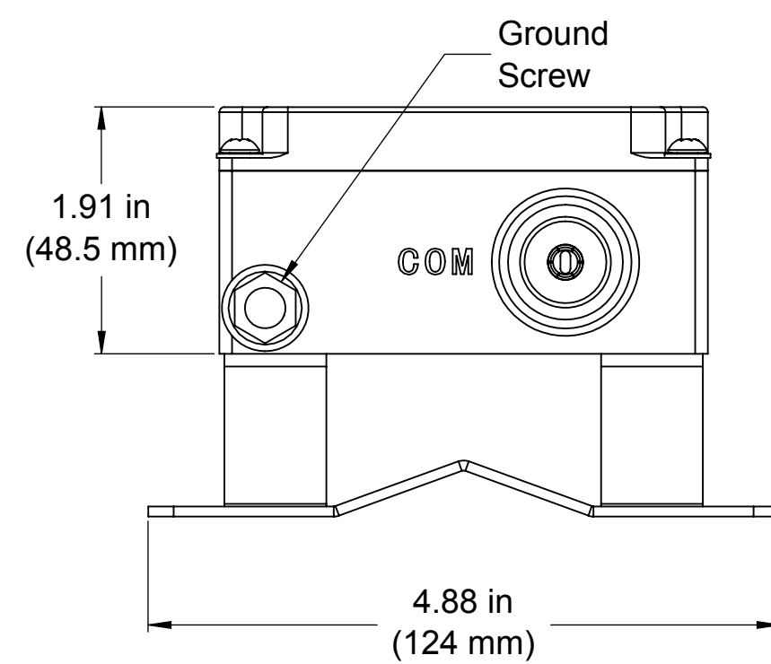
Single diplexer configuration common port view
