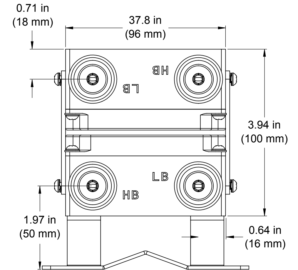
Double diplexer configuration high/low band port view
