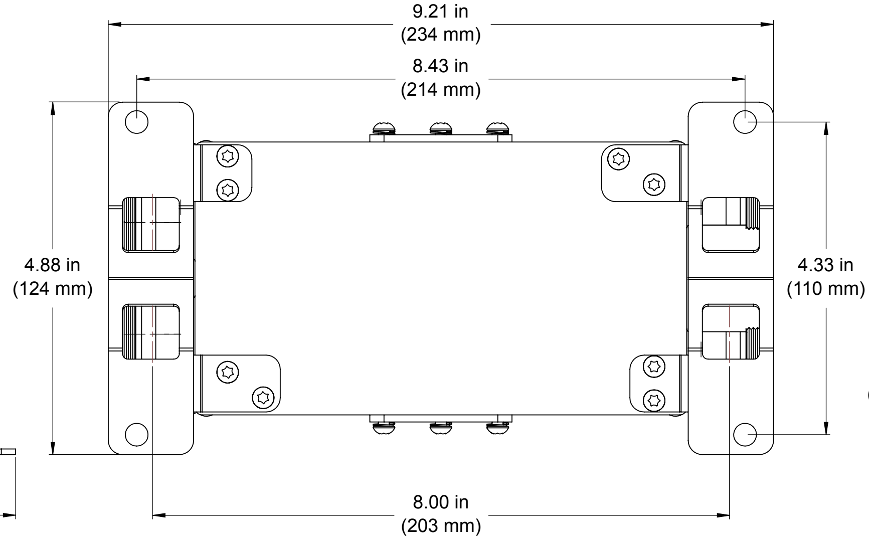
Single diplexer configuration common port view
