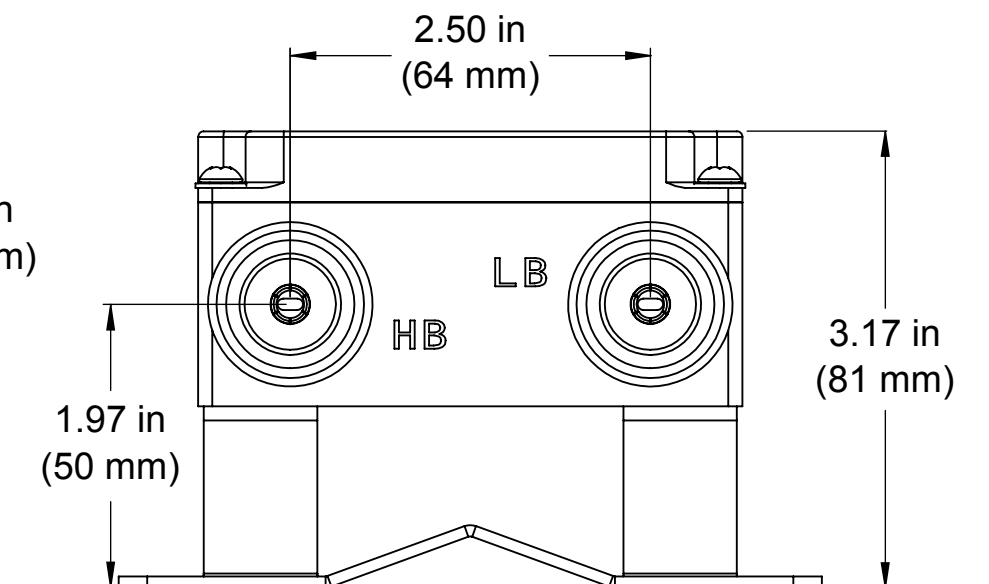
Single diplexer configuration high/low band port view
