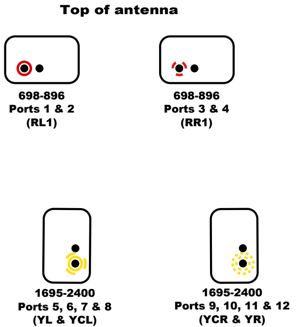
RET placement as viewed from rear of antenna
