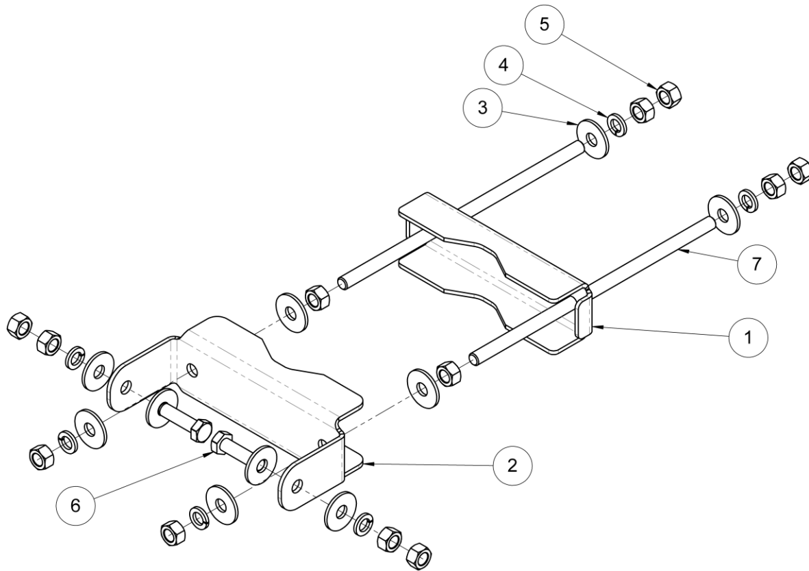
Fig. 2: Fixed Mast Bracket Kit BOM
