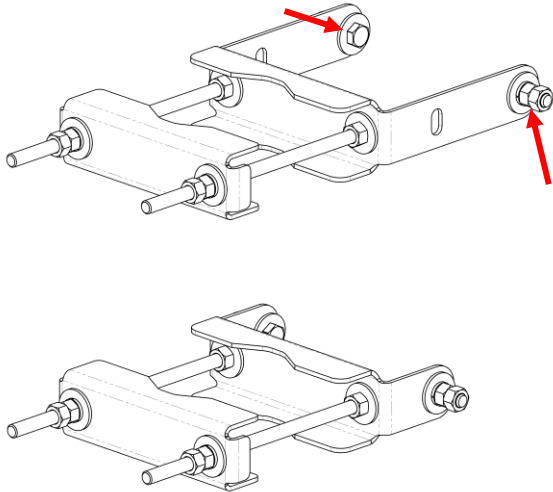
Fig. 3: Dual Position Mast Bracket Hardware Location (at +5° or -5° Tilt)
