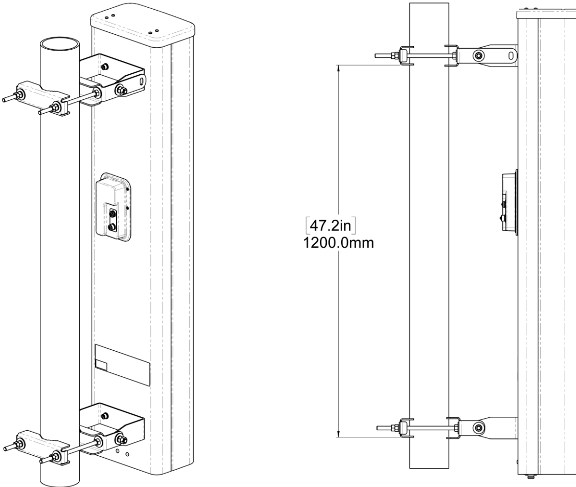
Fig. 7: Dual Position Mast Brackets Attached to the Mast for 0° Mechanical Tilt
