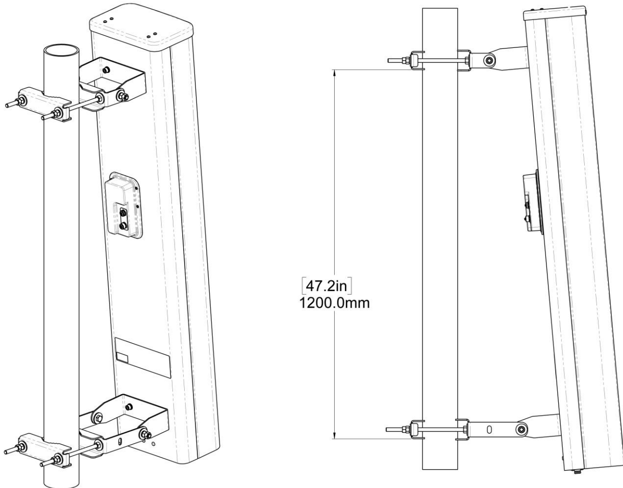
Fig. 8: Dual Position Mast Brackets Attached to the Mast for 5 ° Mechanical Uptilt
