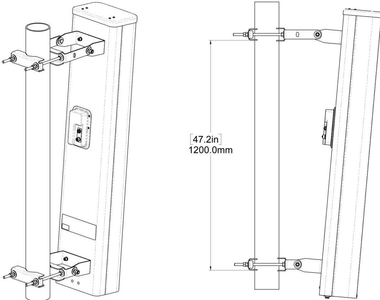
Fig. 6: Dual Position Mast Brackets Attached to the Mast for 5 ° Mechanical Downtilt
