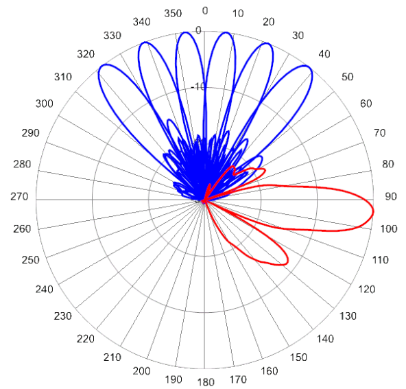
1950 MHz Azimuths with Elevation 4°
