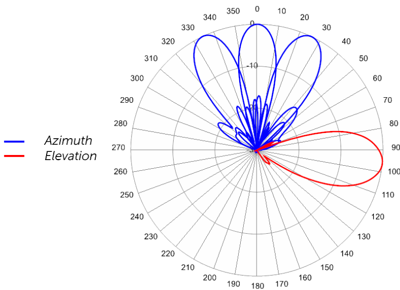
896 MHz Azimuth with Elevation 6°
