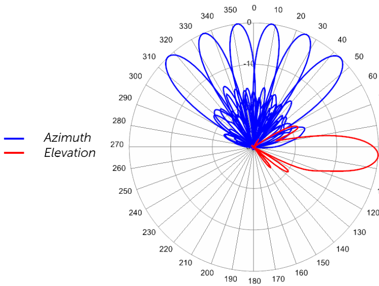
1740 MHz Azimuths with Elevation 4°
