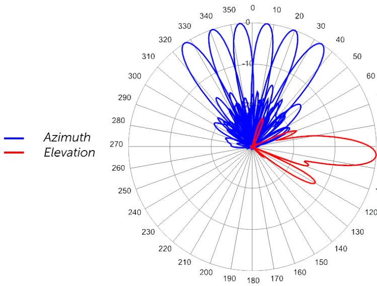
2170 MHz Azimuths with Elevation 4°
