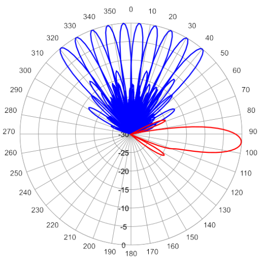
1930 MHz Azimuth / Elevation 4°
