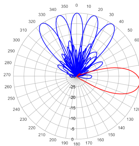
824 MHz Azimuth / Elevation 6°
