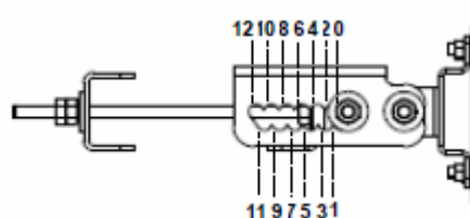
MBK-03 Top Adjustable Bracket Side View
