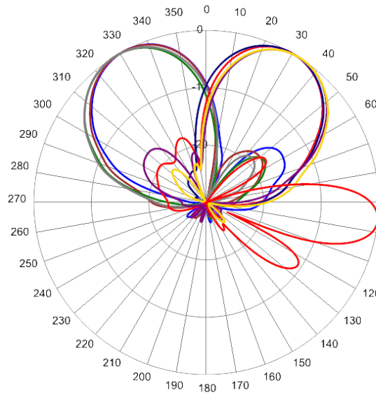
758 MHz Azimuth with Elevation 6°
