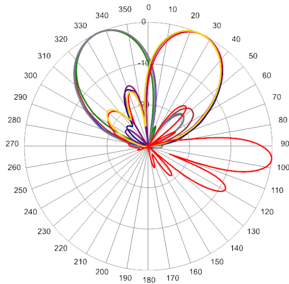
948 MHz Azimuth with Elevation 6°
