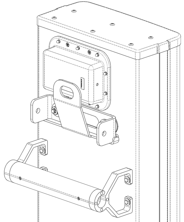
AHH-03 in Hoisting position
