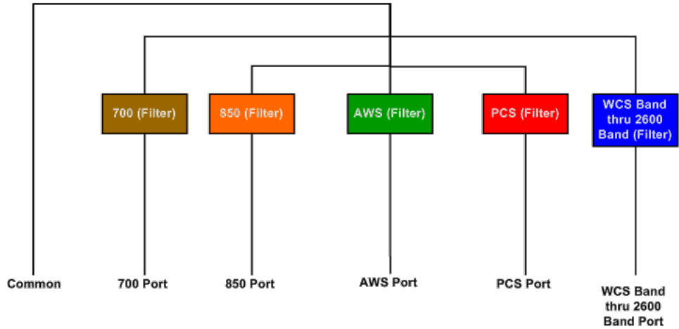
Outdoor Broadband Pentaplexer (5PX-0726-O) Block Diagram
