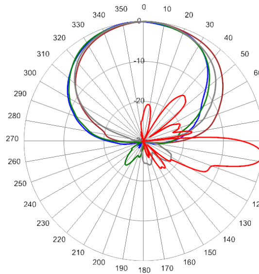
1445 MHz Azimuth with Elevation 7°
