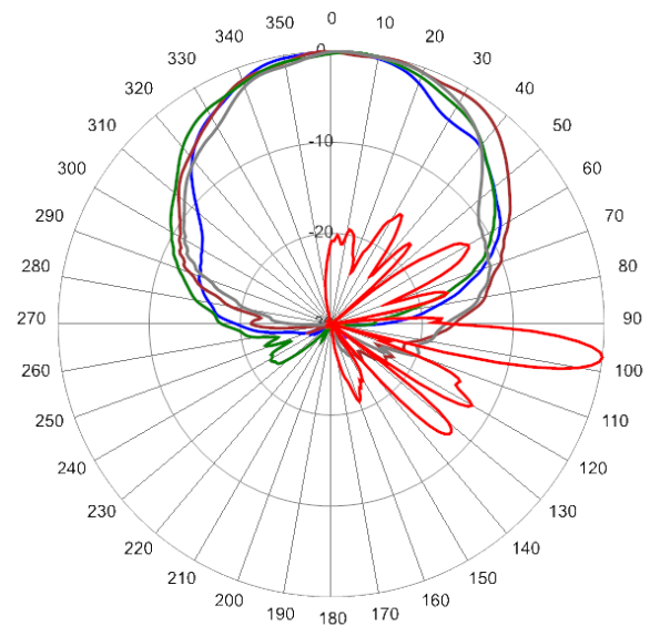
2500 MHz Azimuth with Elevation 7°
