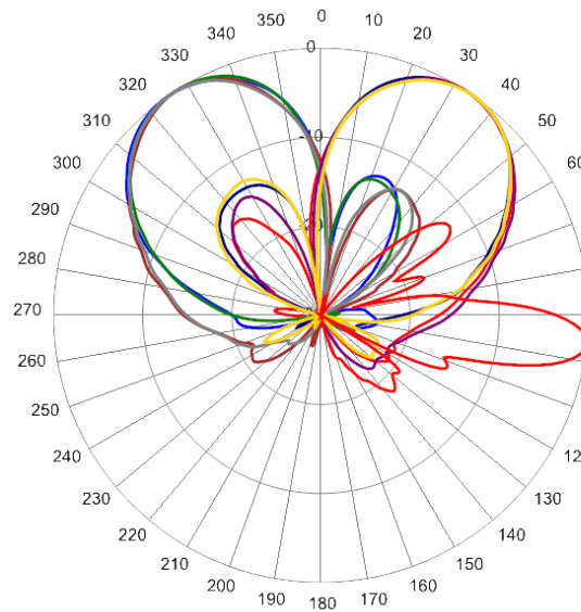
1710 MHz Azimuth with Elevation 6°
