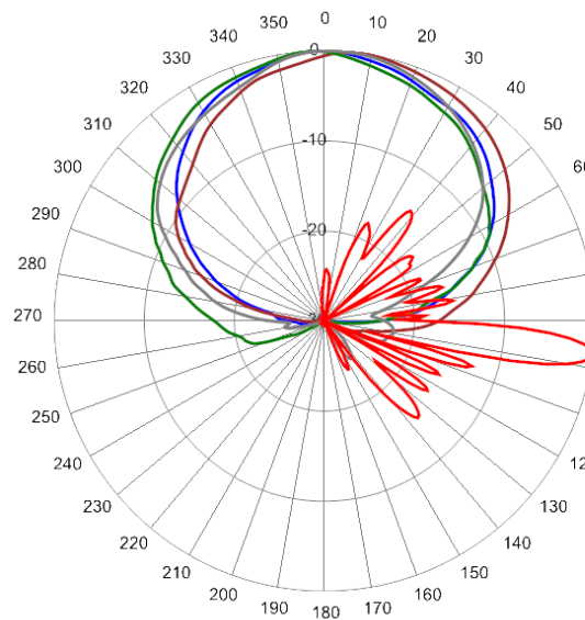
2320 MHz Azimuth with Elevation 7°
